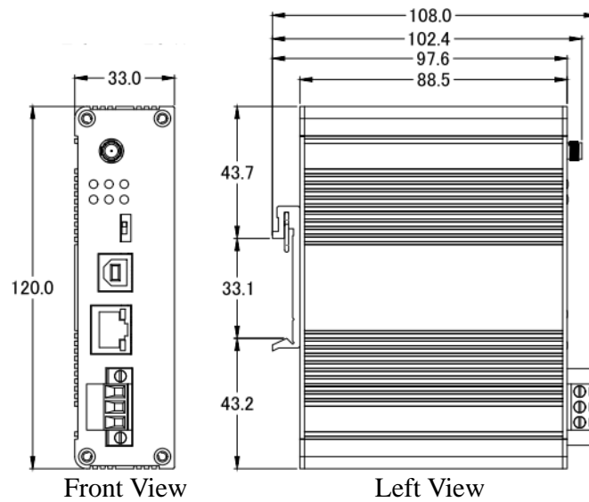
Figure 2-12. Front / Left side dimension of the WF-2572M
