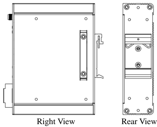
Figure 2-13. Right / Rear side dimension of the WF-2572M
