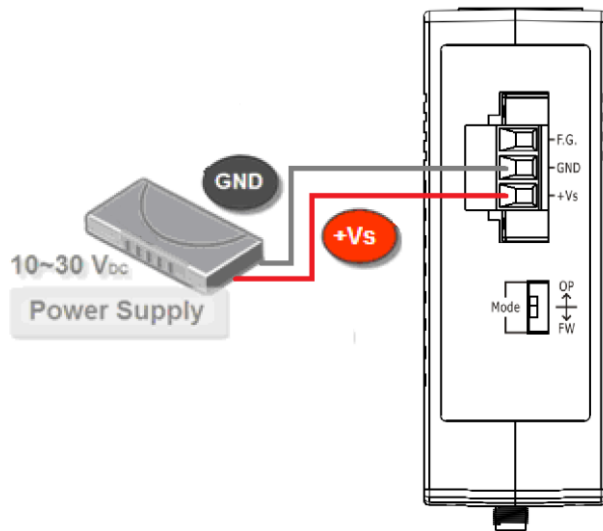
Figure 2-4. Power wire connection of WF-2572
