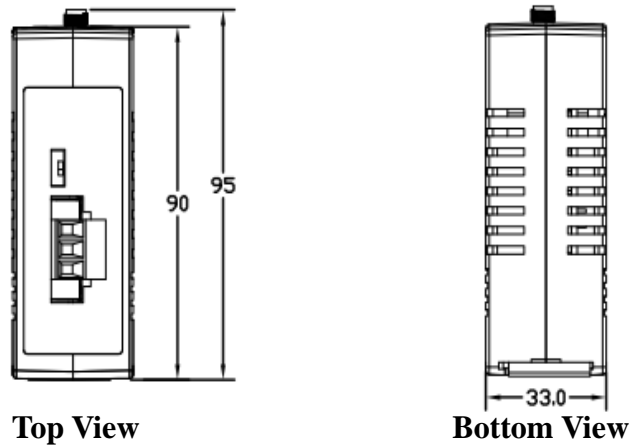
Figure 2-11. Top / Bottom side dimension of the WF-2572
