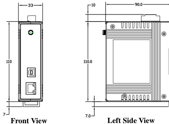
Figure 2-10. Front / Left side dimension of the WF-2572
