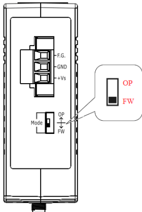
Figure 2-6. FW update position of Dip-Switch
