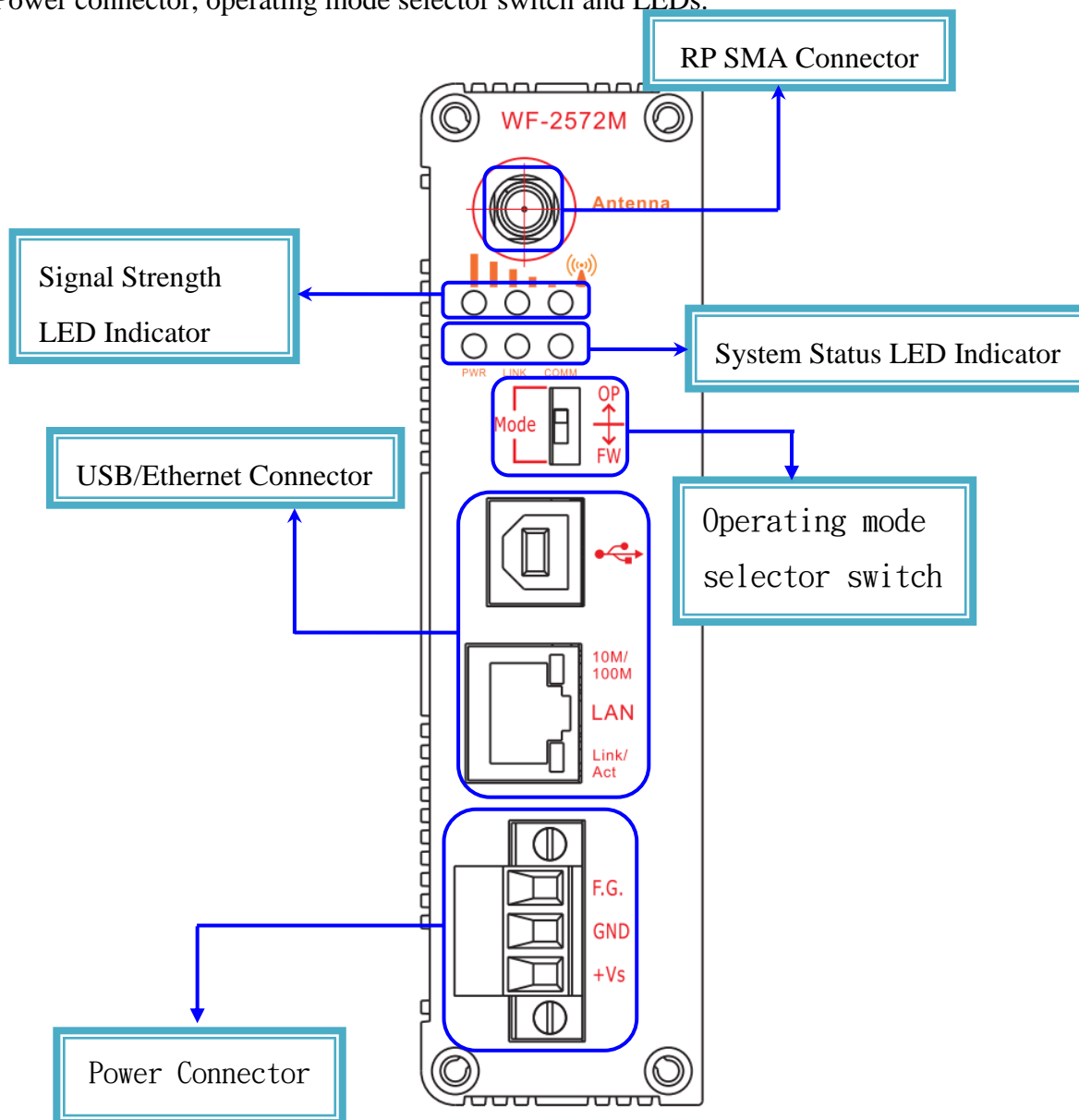
Figure 2-2. Front Panel of the WF-2572
