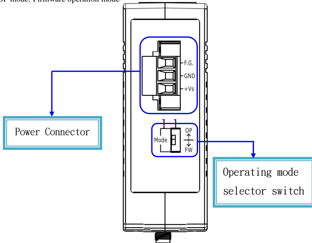
Figure 2-3. Top Panel of WF-2572
