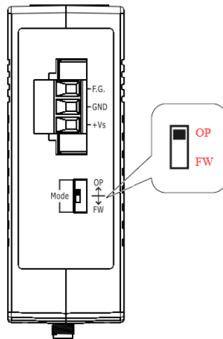
Figure 2-9. OP Position of Dip-Switch
