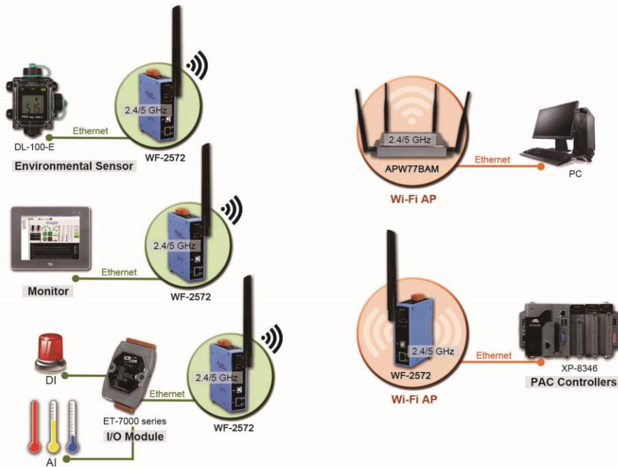
Figure 1-1. The application architecture of WF-2572
